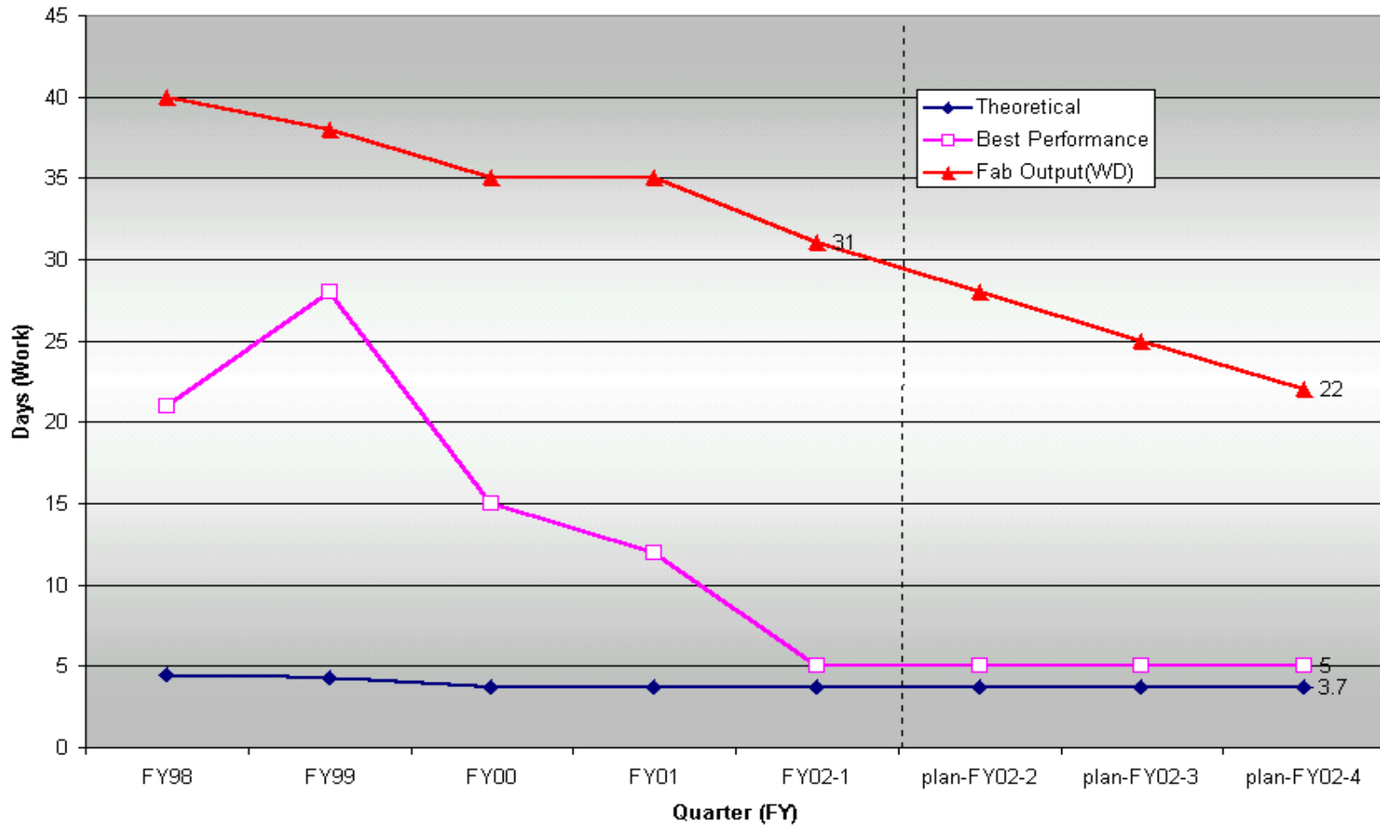
Celeritek Fab Cycle Time
